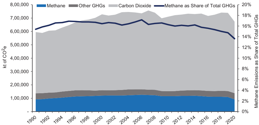
Figure 1: Canada’s 1990 to 2020 greenhouse gas and methane emissions (CO 2 e).
