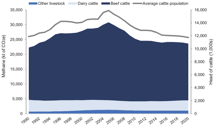
Figure 11: Methane emissions by livestock from enteric fermentation.
