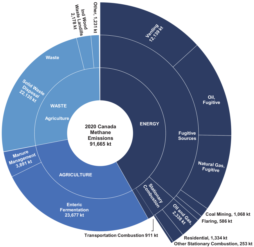
Figure 3: 2020 Methane emissions (kt of CO 2 e) by IPCC subcategory.
