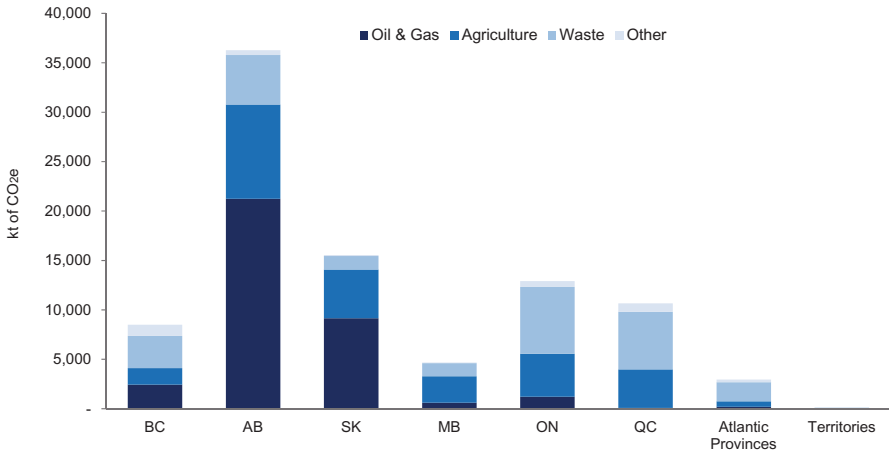
Figure 4: 2020 Methane emissions by province and economic sector.
