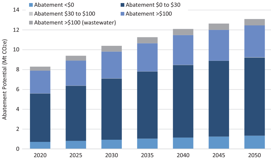
Figure 18: Landfill and wastewater methane abatement potential and costs (USD), 2020–2050.
