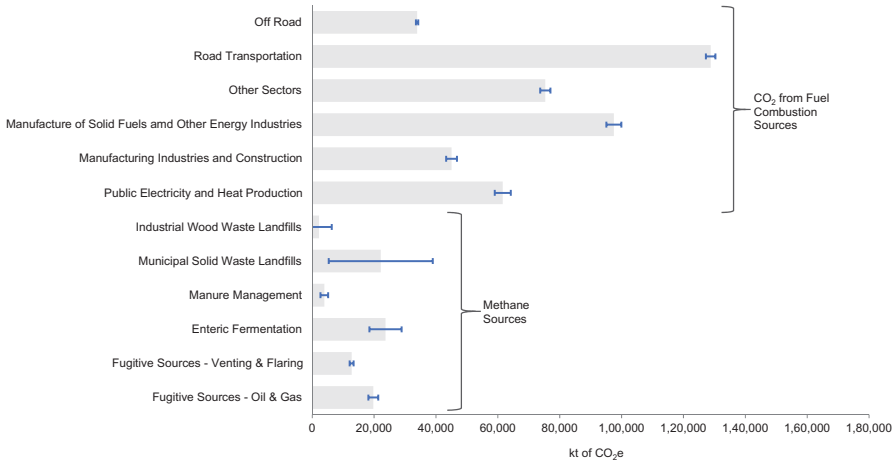
Figure 6: Uncertainty in 2020 NIR emissions estimates.
