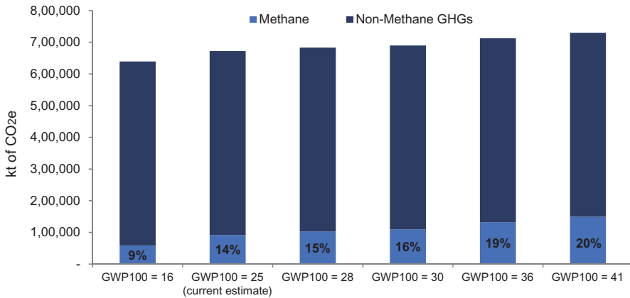
Figure 5: Effect of 100-year methane GWP assumptions on 2020 methane emissions estimate.
