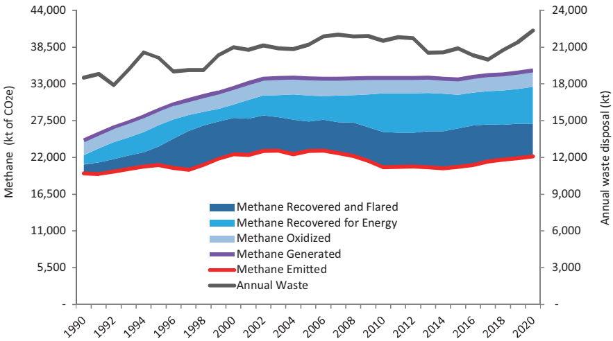
Figure 16: Methane generated from municipal solid waste landfills.
