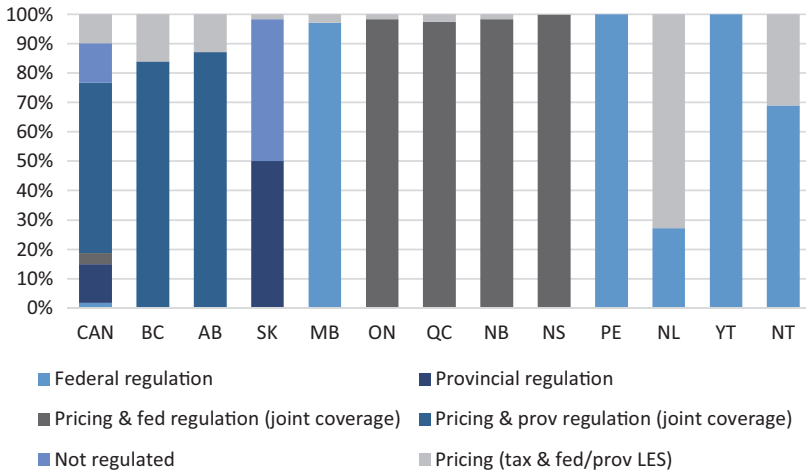
Figure 9: Approximate policy coverage of oil and gas methane emissions by jurisdiction.
