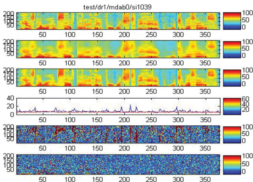
Fig. 3. Top to bottom: Original spectrogram from the test set; reconstruction from the 312-bit VQ coder; reconstruction from the 312-bit auto-encoder; coding errors as a function of time for the VQ coder (blue) and auto-encoder (red); spectrogram of the VQ coder residual; spectrogram of the deep autoencoder's residual.
