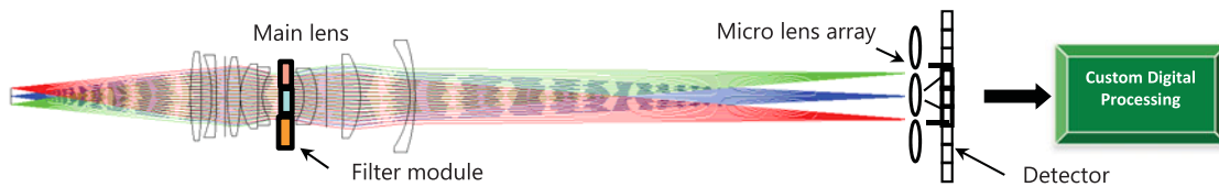
Fig. 3. Basic architecture of multi-spectral light field (plenoptic) imaging [27].
