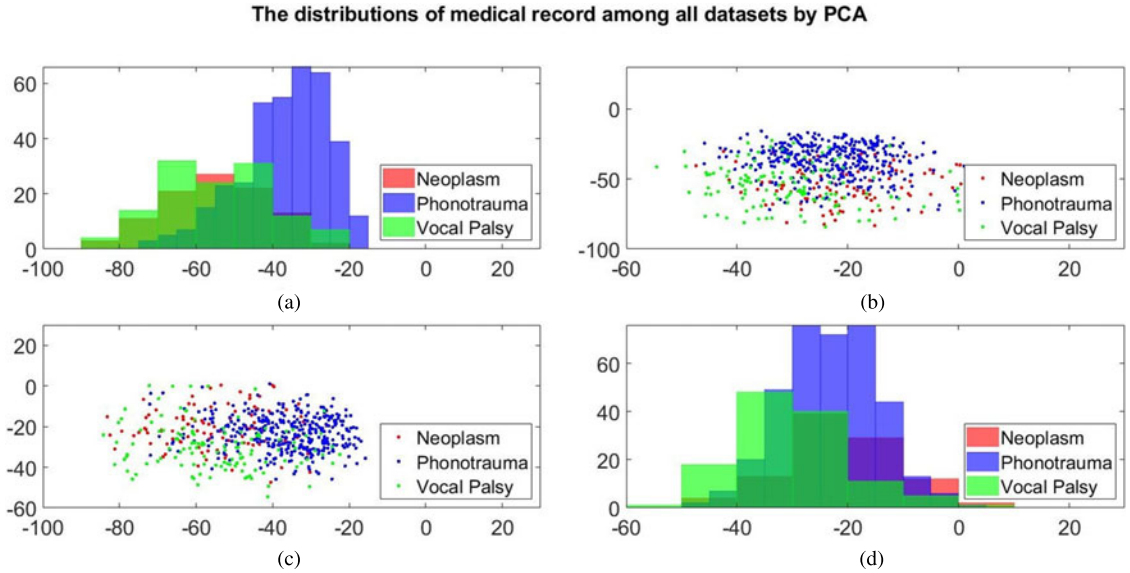
Fig. 5. Distribution of the first and second principal component for medical record. (a) and (d) Are the histogram of individual components, while (b) and (c) are the joint distribution in two-dimension principal component space (the first and second principal components are placed at different axes in (b) and (c)).
