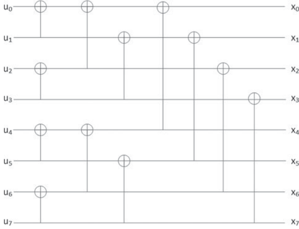
Fig. 7. Encoding of length-8 polar codes.
