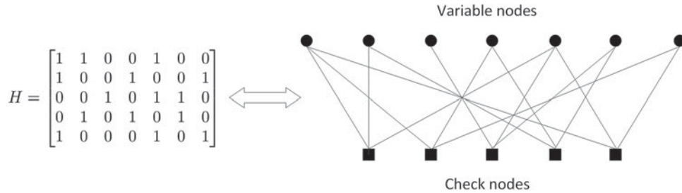
Fig. 1. Graph representation of LDPC parity check matrix.
